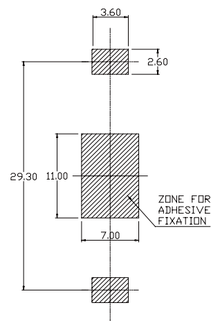
Recommended PCB Layout (PCB TOLERANCE \pm 0.05)
